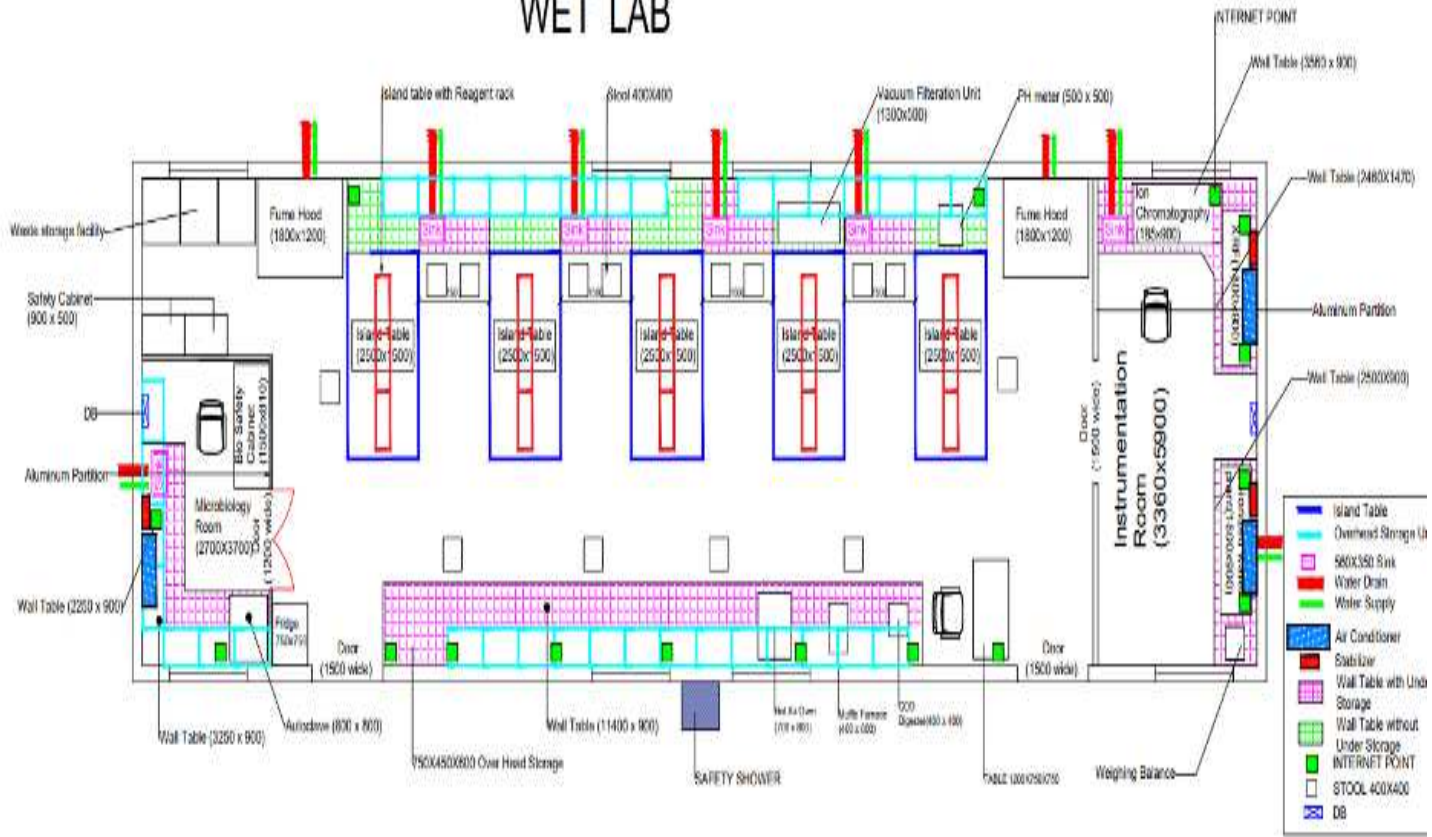
GSCOE WET LAB MODEL LAYOUT FOR FURNITURE
