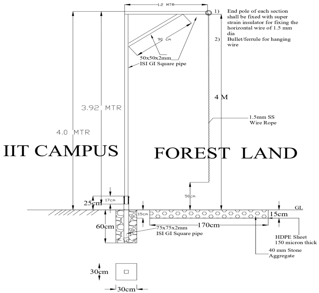
FIG 1: TYPICAL ARRANGEMENT FOR NO COMPOUND WALL AREA. NECESSARY WORK FOR POSITIONING THE POLE SHALL BE MADE ON THE GROUND DEPENDS UPON SITE CONDITION.
