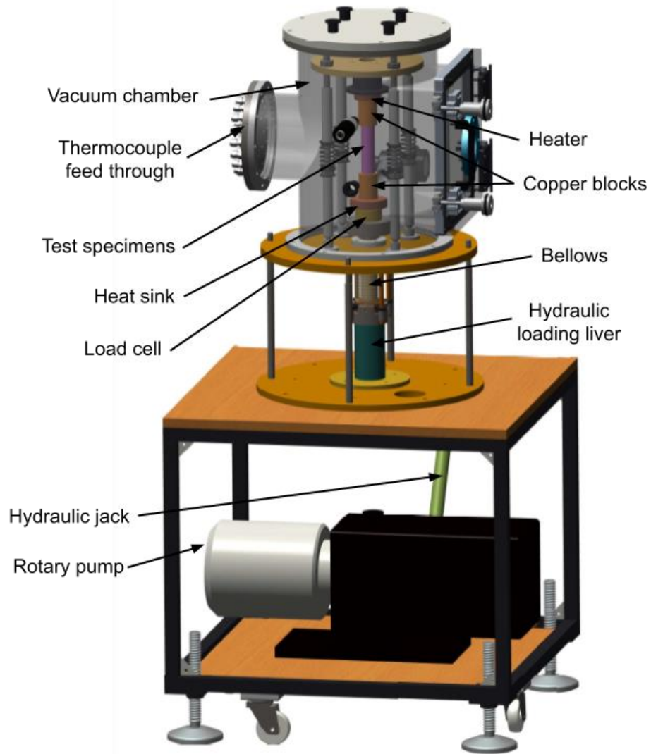
Fig. 1: Uniaxial loading setup with customized vacuum chamber
