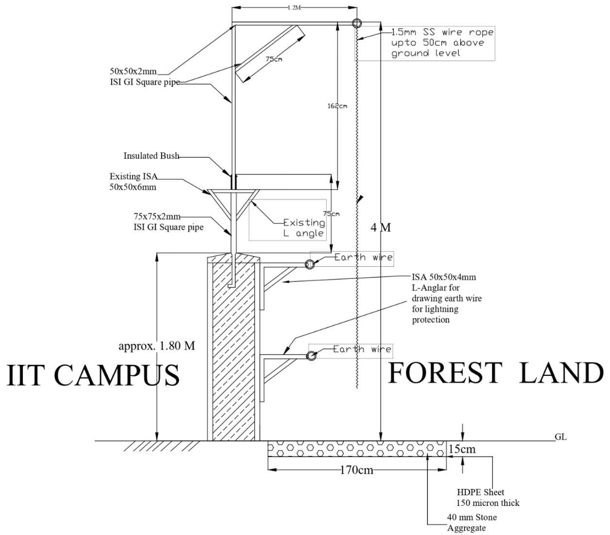
FIG: 2 TYPICAL LAYOUT FOR SOLAR FENCING
